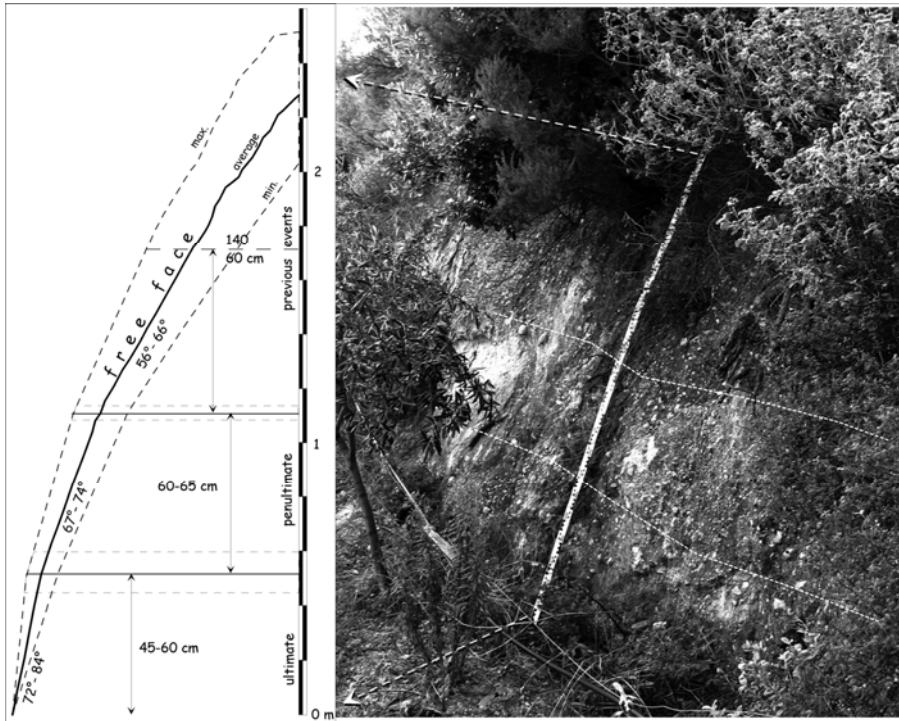
Figure 16. Free-face cropping out at the base of the Rossano Fault scarp (location in Fig. 5), and, on the left, sketch summarizing the geometrical properties of the plane (dips and heights have been averaged on twelve spaced sections). We recognized at least three ~0.6-m-high bands with different dip and degradational aspect, each one partly associable to single coseismic rupture. The upper (and oldest) one is deeply degraded, and it presents the lowest dip; thus, it might record several past surface ruptures, beside long-term erosive exhumation.
