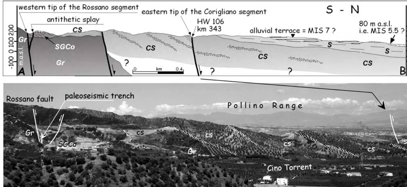
Figure 7. Simplified geological cross section across the Rossano Fault (A-B in figure 6; legend same as figure 6). The section shows the overlap zone between the Corigliano and Rossano segments. Note the Middle(?) Pleistocene marine succession, dipping seaward, faulted against the crystalline Sila basement. The possible inner-edge of the marine terrace MIS 5.5 is shown. The lower panel is a picture of the left sector of the geological sketch.
