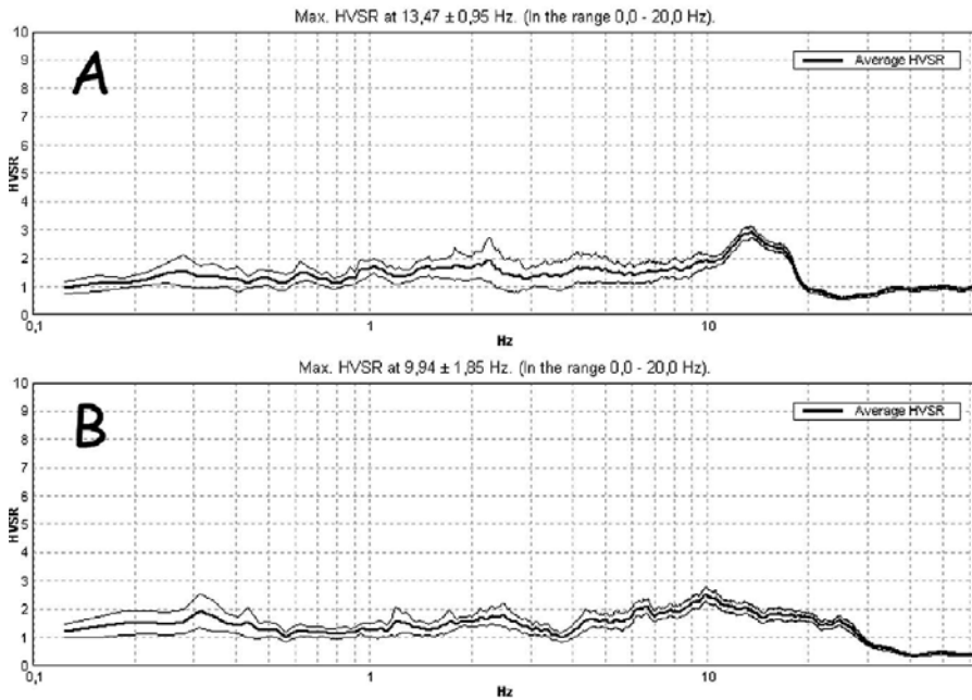
Figure 3. HVSR obtained in Rossano (A) and Crosia (B). Note the absence of amplification for any frequency. This fact has been observed in all the villages where we performed microtremor analyses.
