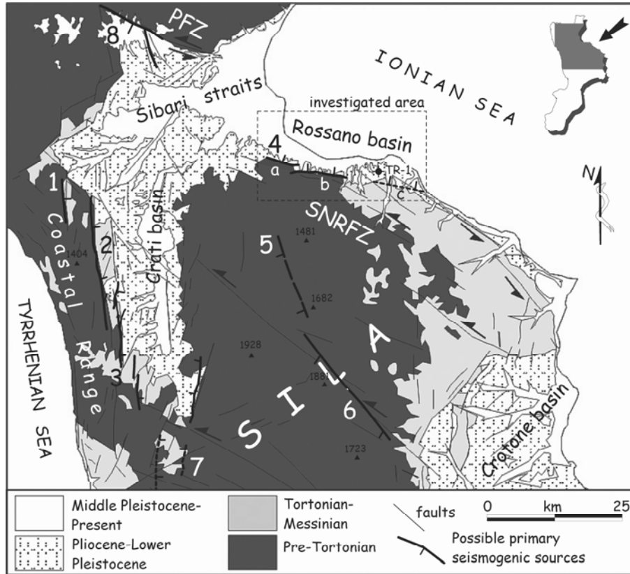
Figure 4. Structural sketch of northern Calabria and main possible seismogenetic faults: 1-3, W-Crati Fault System (1, Fagnano-Castello; 2, San Marco-San Fili; 3, Montaldo-Rende); 4, Rossano (segment a: Corigliano; b, Rossano; c, Crosia); 5, Cecita Lake; 6, Lakes; 7, Piano Lago-Decollatura; 8, Mt. Pollino. PFZ (Pollino Fault zone) and SNRFZ (S. Nicola-Rossano Fault zone) represent crustal shear zone. Only faults 4, 6, and 8 have been studied by means of paleoseismological analyses. TR-1, Trionto 1 borehole.
