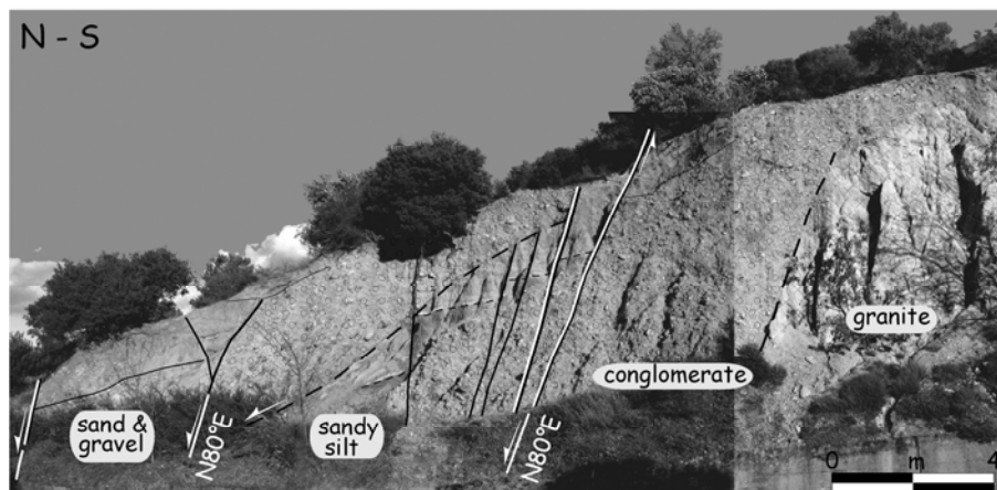
Figure 9. View looking east of the western tip of the Rossano Fault zone (location in figure 5). The Middle Pleistocene fan-delta succession (conglomerates and sandy silts and gravels, partly laying over the granite basement; right side) is displaced by several ~E-W normal faults. These faults downthrow definitely the Sila Massif below the coastal plain (left side), where the crystalline bedrock has been reached in borehole at 1600 m below s.l.
