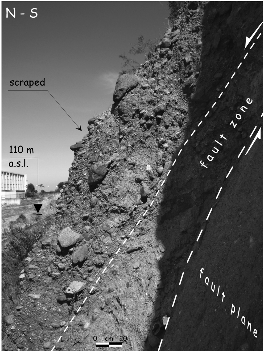
Figure 11. View looking west of one of the faults affecting the flight of marine/alluvial terrace close to the Rossano town (location in figure 5). Note the clasts of the terrace deposits dragged along the fault zone.
