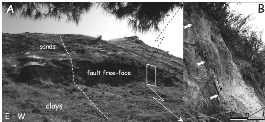
Figure 15. Morphological evidence of the recent fault re-activation (location in Fig. 5). A) view looking south of the fault scarp affecting the Middle Pleistocene sandy-clayey succession near Corigliano. Considering the high erodibility of these terrains, the freshness of the scarp suggests a recent activity of the fault. B) fault-plane (arrows) along the same scarp, between the marine sands (footwall) and talus and marine clays in the hangingwall.
