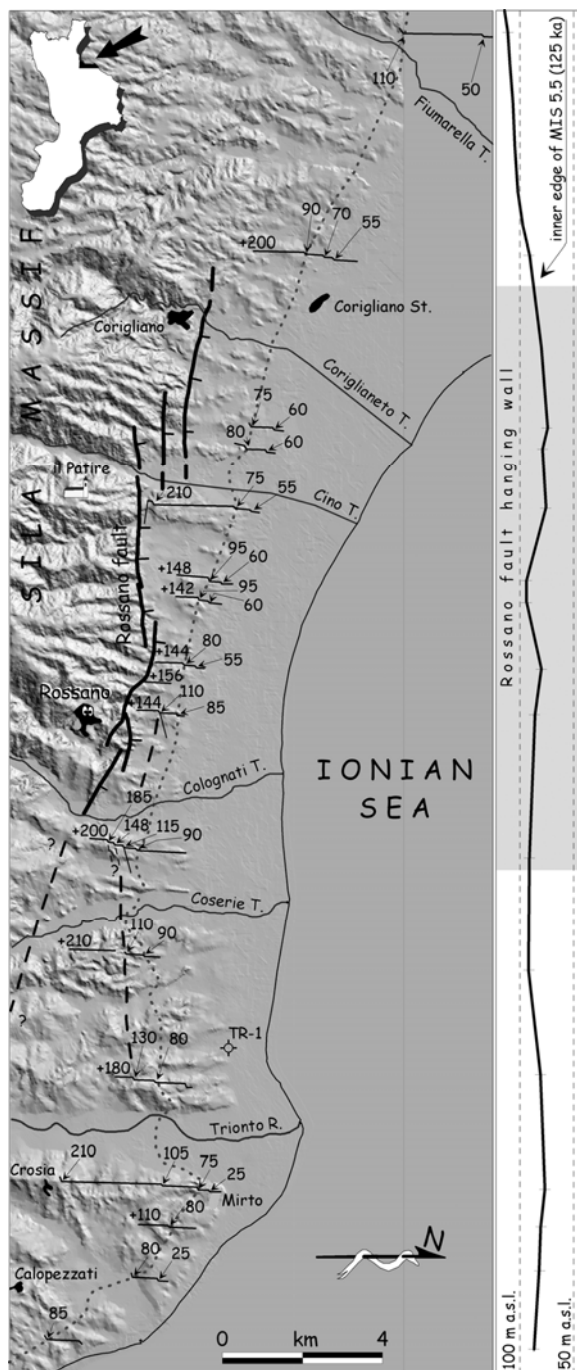
Figure 10. Shaded relief image of the Rossano coast. The main segments of the Rossano Fault are shown, together with seventeen topographical sketches drawn across the flight of marine/alluvial terraces of the area. Elevations in meters a.s.l. refer to the bottom of each identified scarp (arrows) that – in case of marine terrace – should indicate the inner edge of the relative MIS. Certain fault-scarps are evidenced on the sections by a line dipping seaward (dashed where inferred). Elevations marked by the symbol + indicate that the surface has not a scarp uphill. The right panel shows the projected profile of the presumed MIS 5.5 coastline, which appear lowered by the Rossano Fault with respect to the western (top) area.
