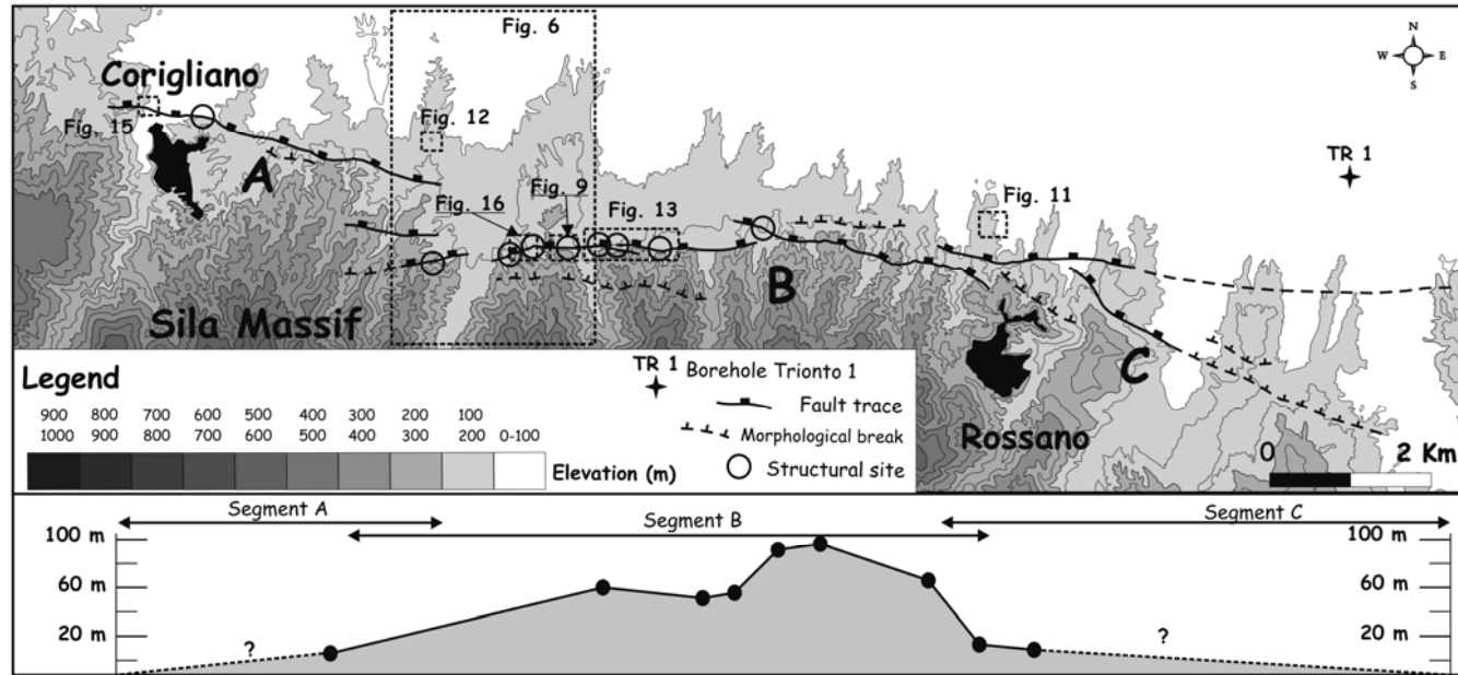
Figure 5. Rossano Fault segments (a=Corigliano segment, b=Rossano segment, c=Crosia segment) and locations of the structural sites and figures. TR-1 is the location of the deep borehole Trionto 1, reaching the crystalline basement at ~1600 m below s.l. In the figure is also shown the distribution along fault of the scarp height.
