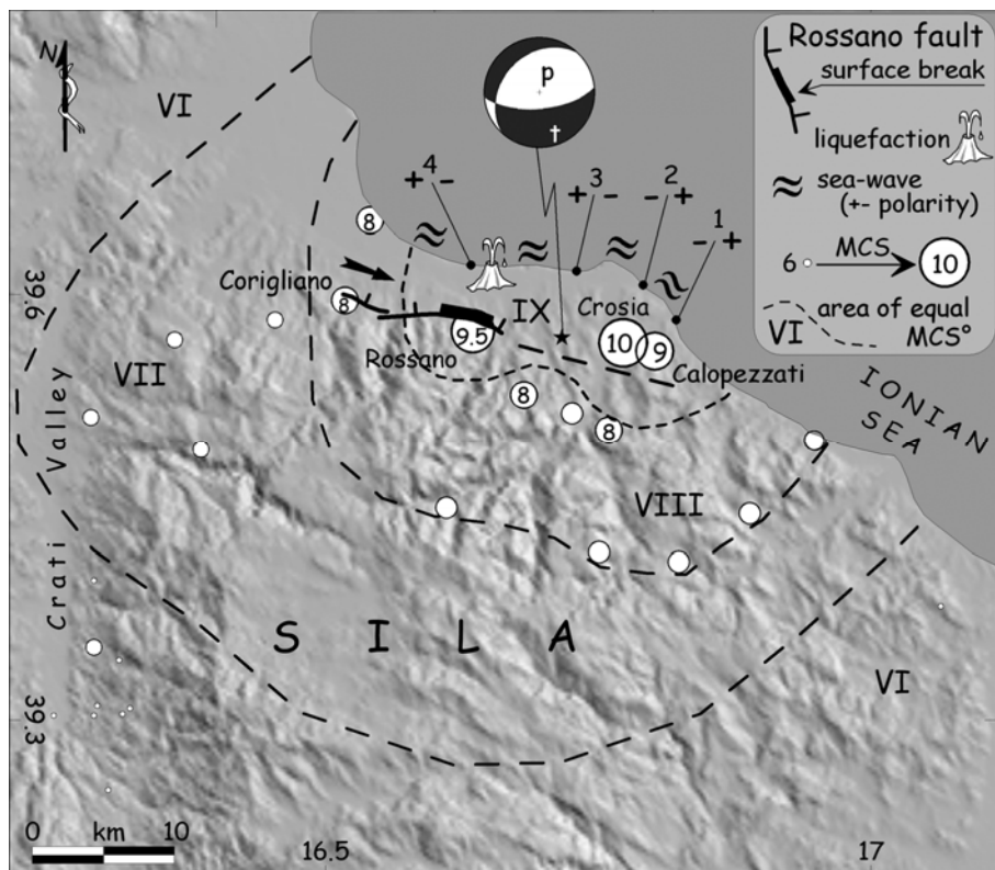
Figure 2. Intensity distribution of the 1836 earthquake. Note that the isoseismic lines are opened seaward, and that the mesoseismic area roughly parallels the Rossano Fault; this fact suggests that this fault could be associated with the 1836 seismogenic structure. The tsunamis effects along the coast (site 1, Caloveto beach; 2, Centofontane; 3, Iapichello; 4, Sant'Angelo; from Rossi, 1836; De Rosis, 1838) imply the occurrence of a coseismic deformation of the area; polarity might indicate the lowering in the nearfield of the Rossano Fault hangingwall (positive, sea ingression), with sea retreat in the surrounding zones (negative). The black arrow indicates the possible fault rupture direction, accounting for strong effects in the small villages of Crosia and Calopezzati. The focal mechanism refers to the M_L=3.4 earthquake of December 02, 1995 (Vannucci and Gasperini, 2004; p, P-axis; t, T-axis).
