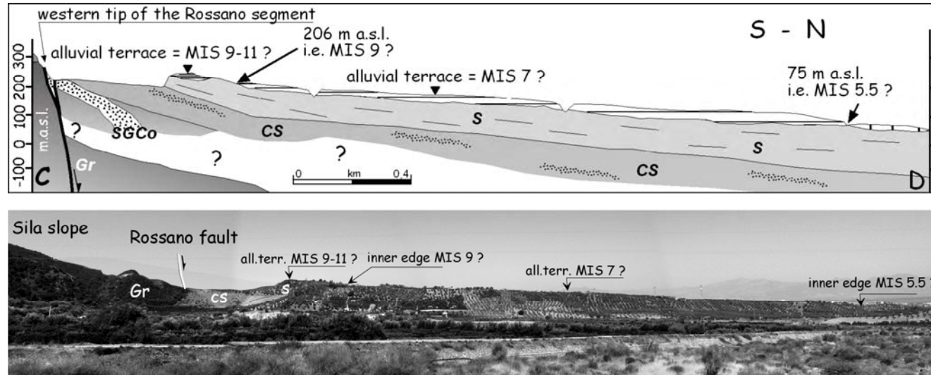
Figure 8. Simplified geological cross section across the Rossano Fault (C-D in figure 6). Note in this section the flat paleosurface topping the Pleistocene sands (S), tentatively interpreted as an alluvial coastal plain terrace, developed over a previous marine erosional terrace. The possible inner-edge of this marine terrace (MIS 9) is showed, together with the one of MIS 5.5. Lower panel is a picture of the geological sketch.
