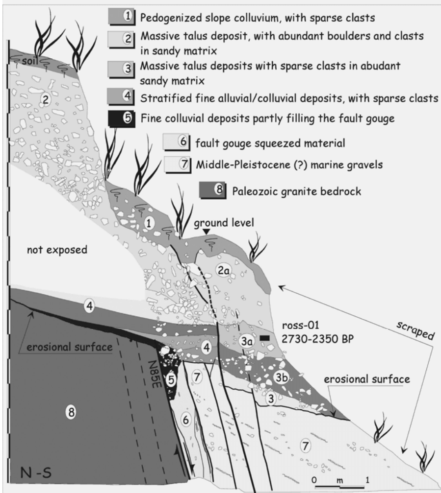
Figure 17. Sketch of the paleoseismic trench excavated across the Rossano Fault (location in Fig. 6). Even if no certain event-horizons can be recognized within the talus succession, the absolute age of a charcoal sampled in unit 3 provides the terminus post-quem for the latest fault ruptures.
